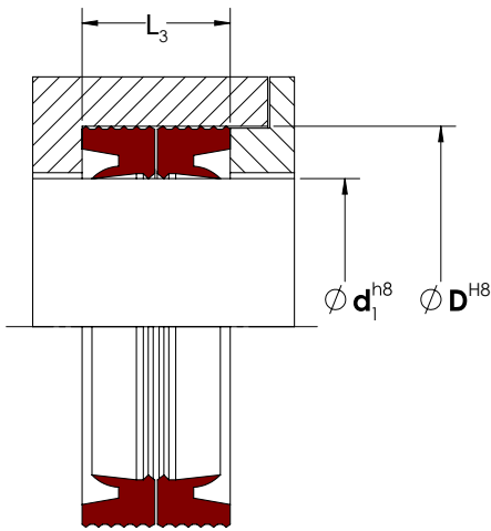
BACK-TO-BACK CONFIGURATION
